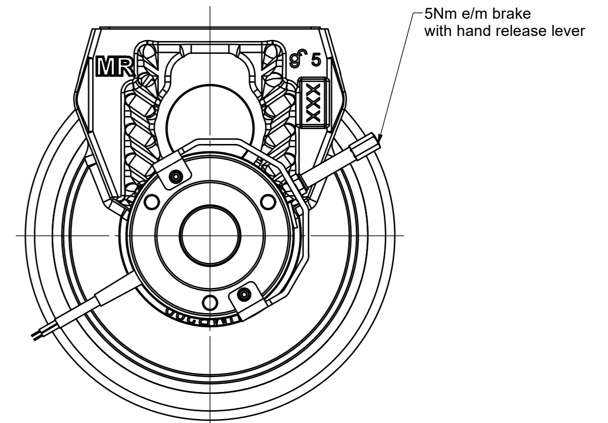
View from "A"
