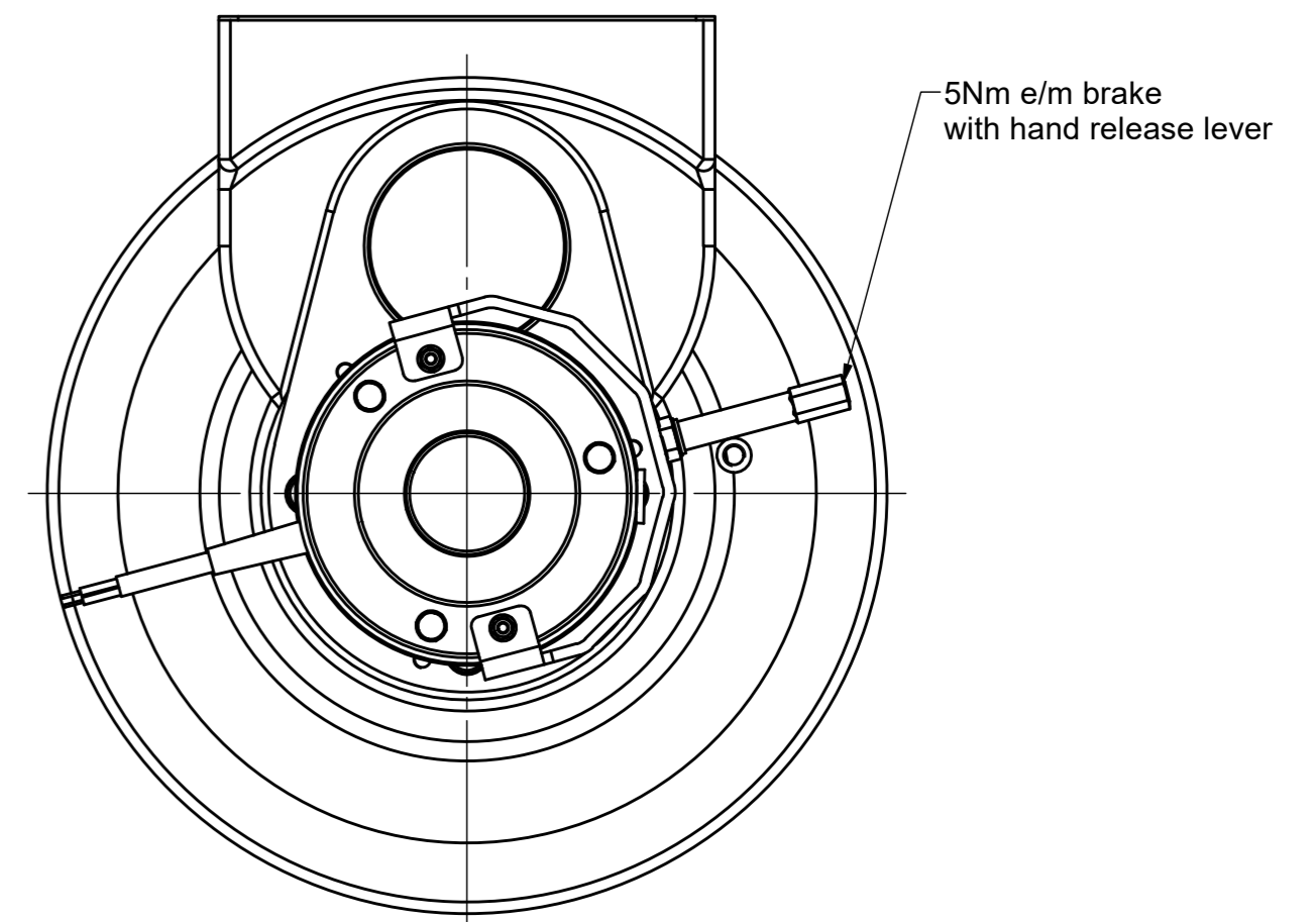
View from "A"
