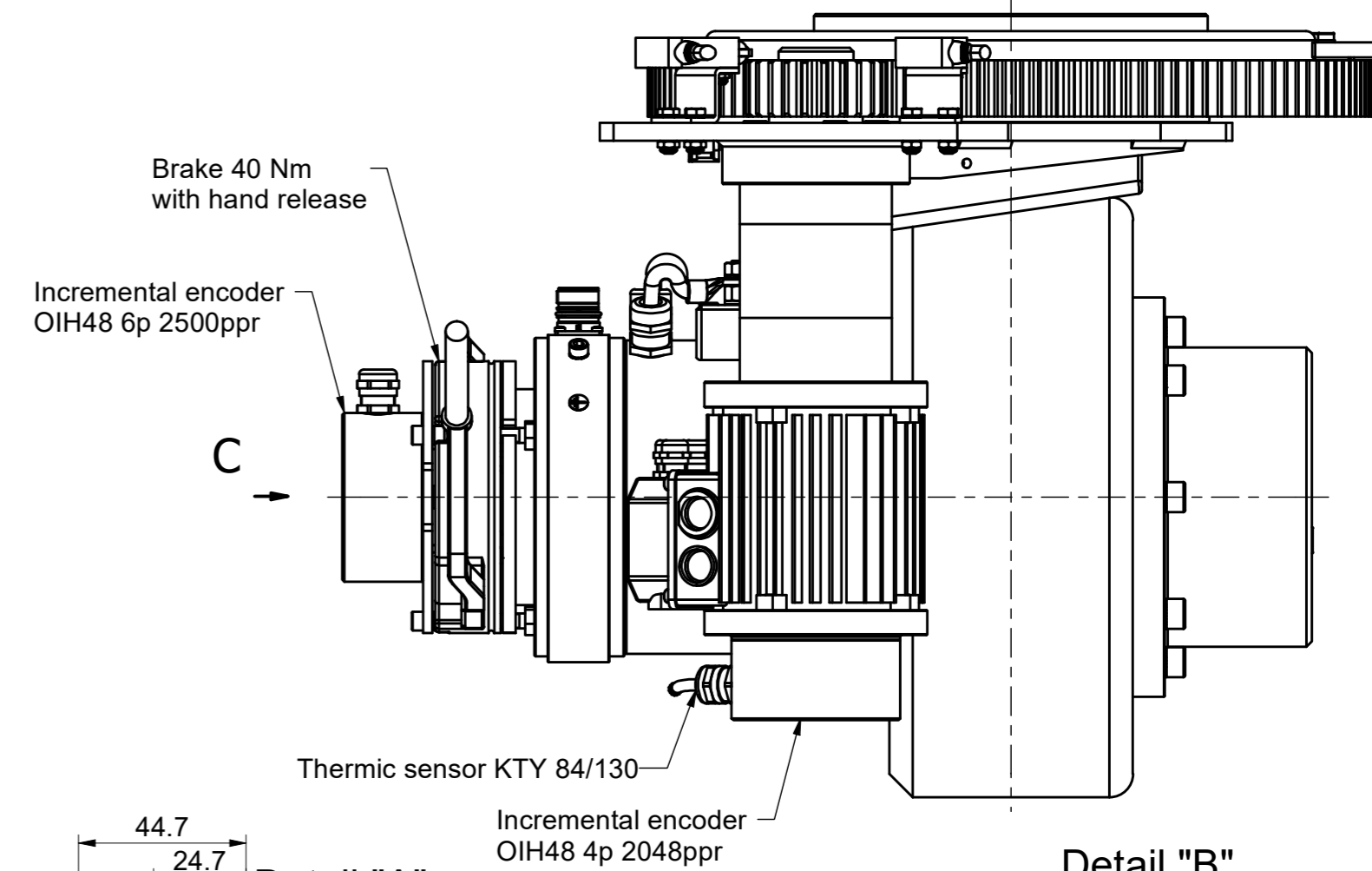
Detail "A"
