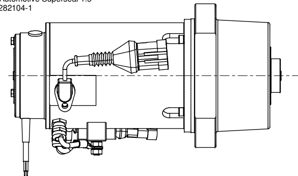
Thermal sensor KTY 84/130 Plug AMP Automotive Superseal 1.5 Series P2 282104-1
