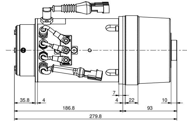
Radial sensor 32 PPR Plug AMP Automotive Superseal 1.5 Series P4 282106-1
