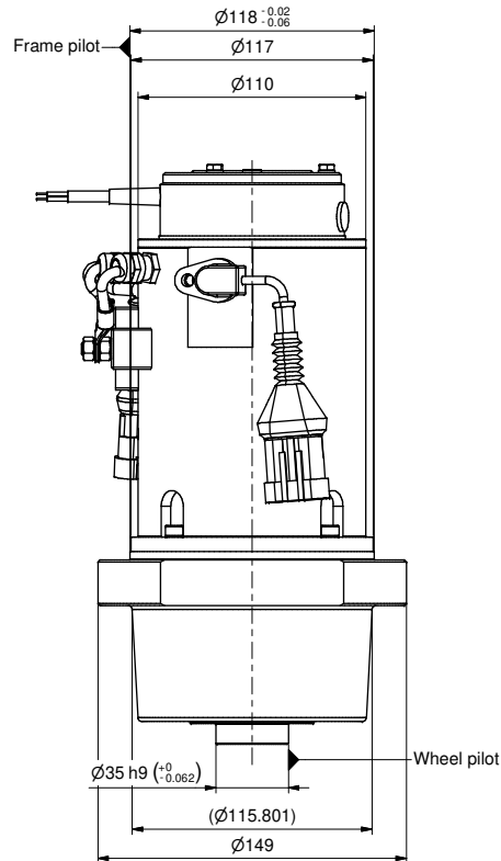
Thermal sensor KTY 84/130 Plug AMP Automotive Superseal 1.5 Series P2 282104-1
