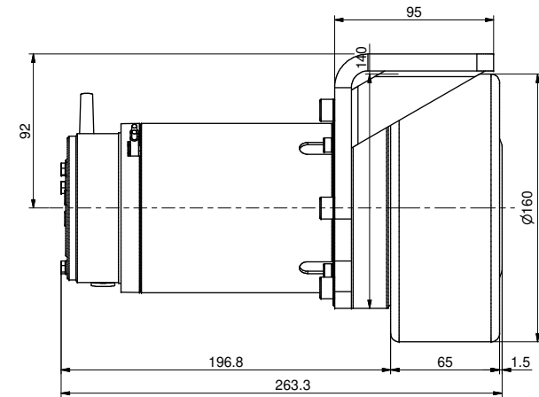
View with wheel and frame plate
