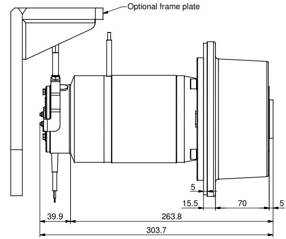
View with wheel and frame plate
