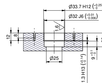
Sec. B-B
