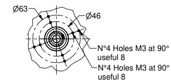
Detail D
