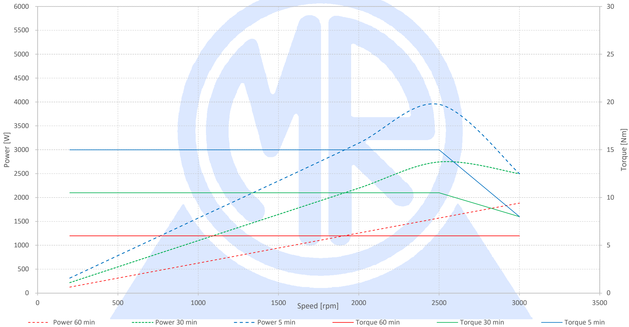
Duty Cycle Curve PSFBL73
