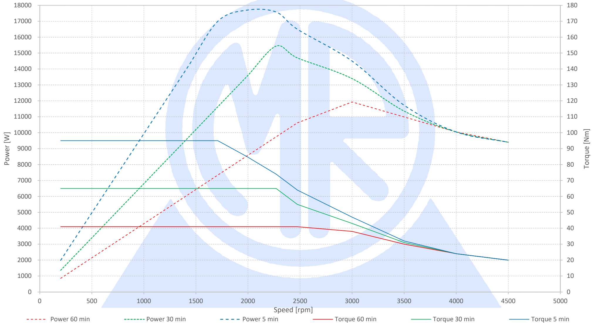
Duty Cycle Curve PSF15
