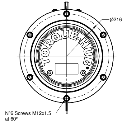
Radial sensor 48 PPR Plug AMP Automotive Superseal 1.5 Series P4 282106-1
