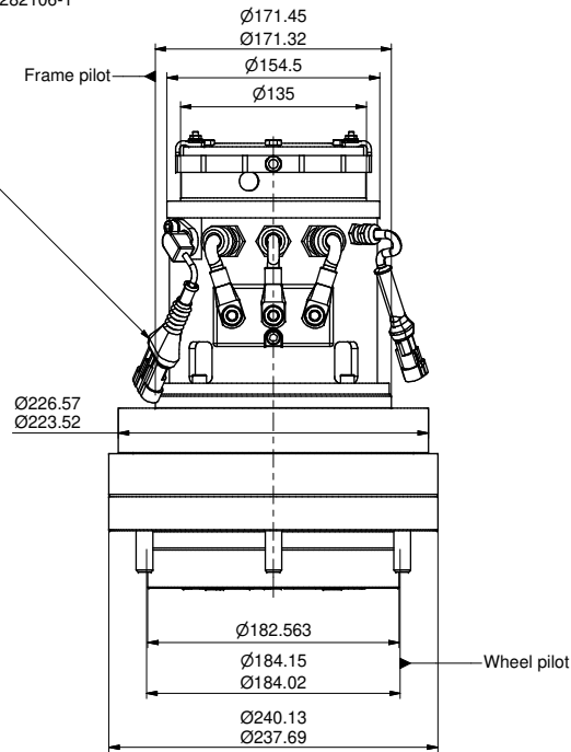
Radial sensor 48 PPR Plug AMP Automotive Superseal 1.5 Series P4 282106-1
