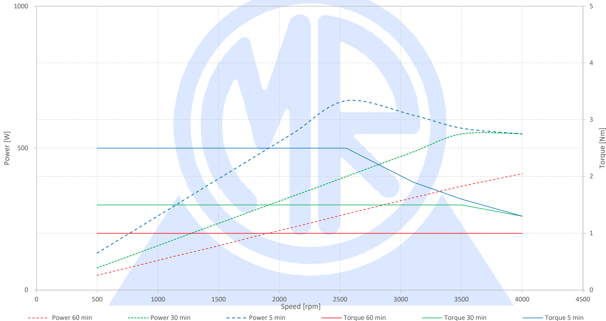
Duty Cycle Curve PSFARD104
